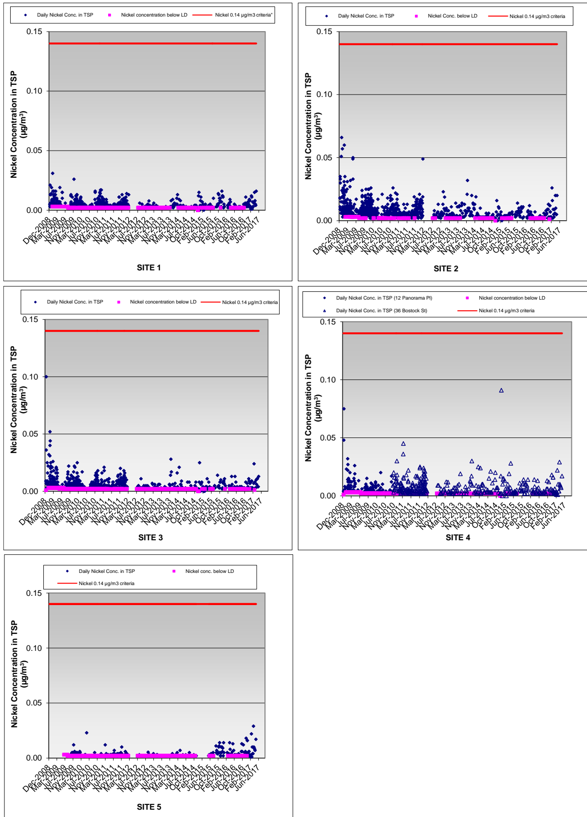
Figure 1: Concentrations of Nickel measured in Total Suspended Particulate (TSP) by High Volume Air Samplers (HVAS) at Sites 1 to 5 from 12 th December 2008 to 10 th May 2017
