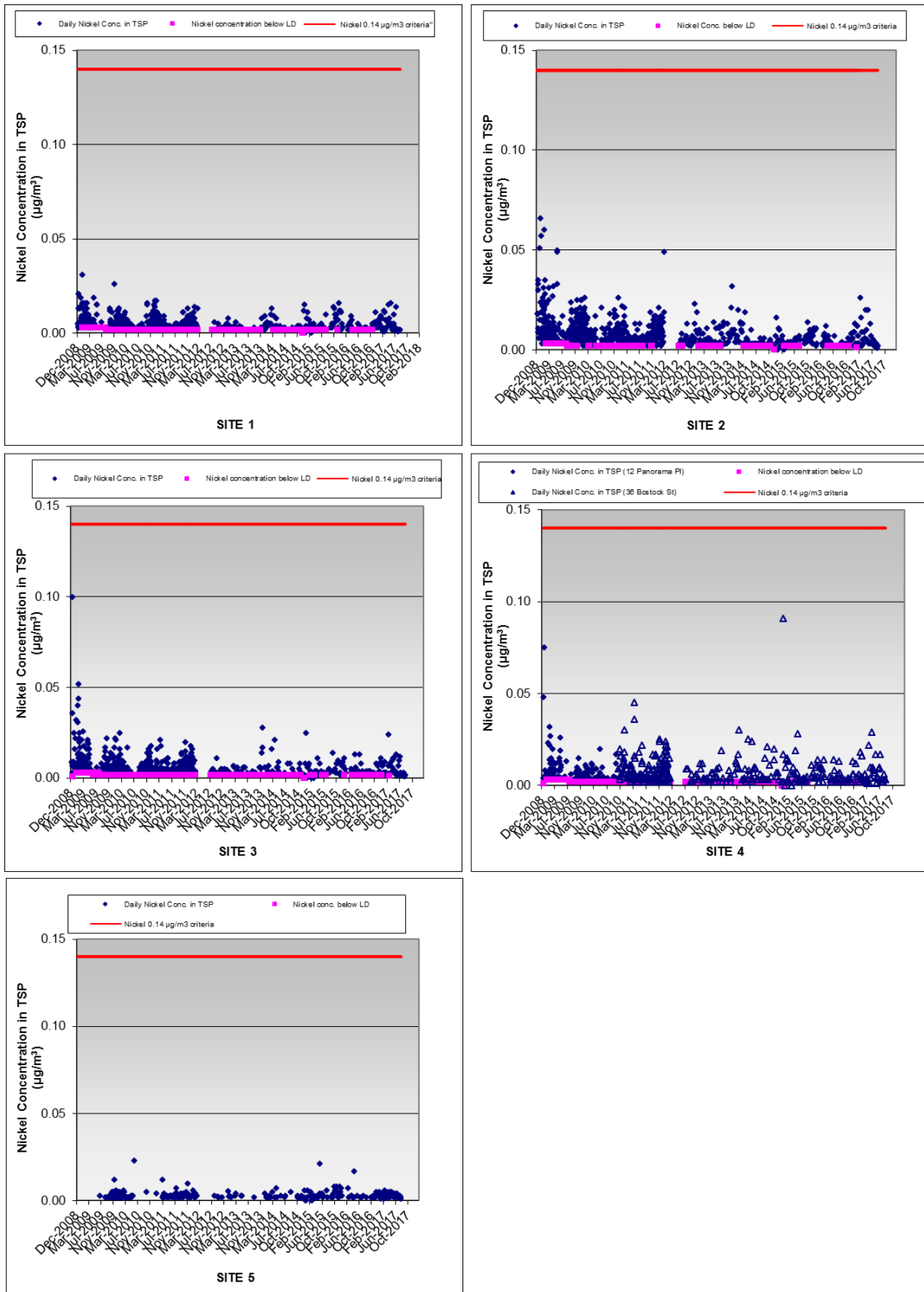
Figure 1: Concentrations of Nickel measured in Total Suspended Particulate (TSP) by High Volume Air Samplers (HVAS) at Sites 1 to 5 from 12 th December 2008 to 8 th August 2017
