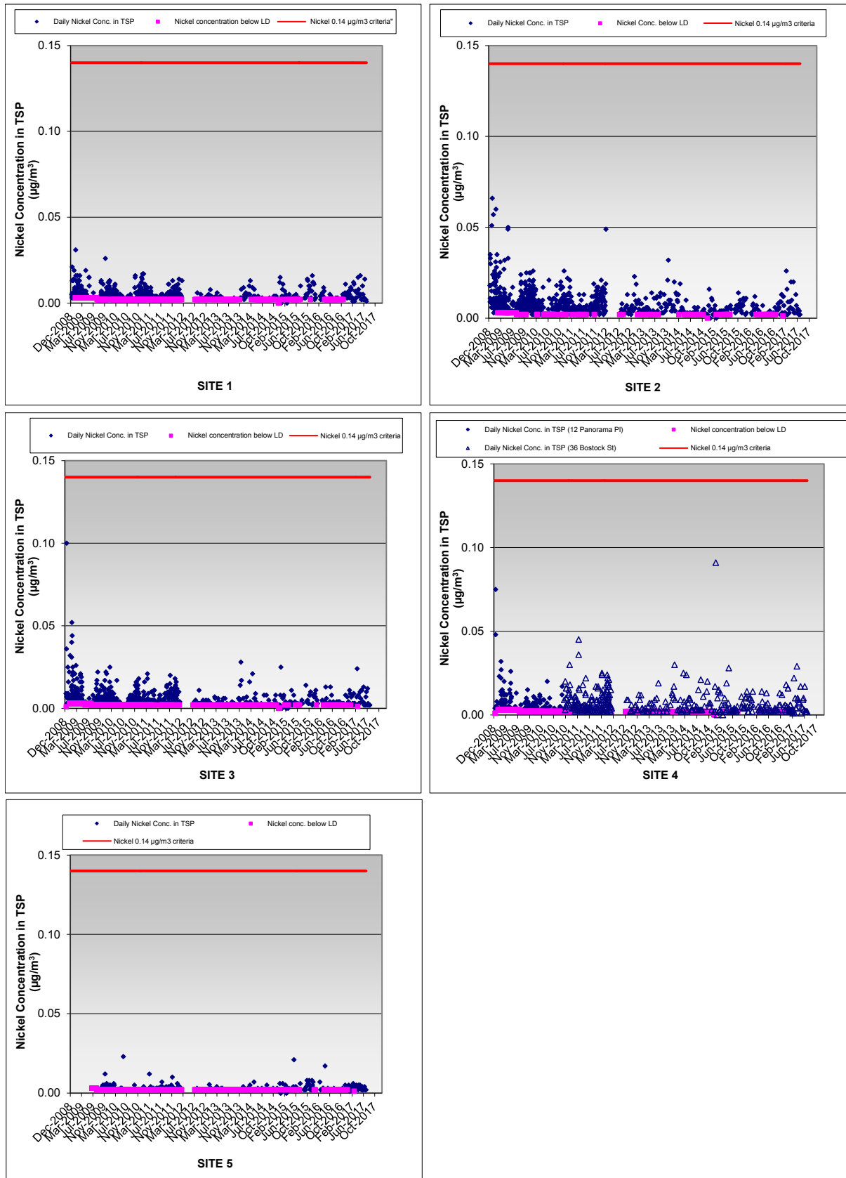
Figure 1: Concentrations of Nickel measured in Total Suspended Particulate (TSP) by High Volume Air Samplers (HVAS) at Sites 1 to 5 from 12 th December 2008 to 15 th July 2017
