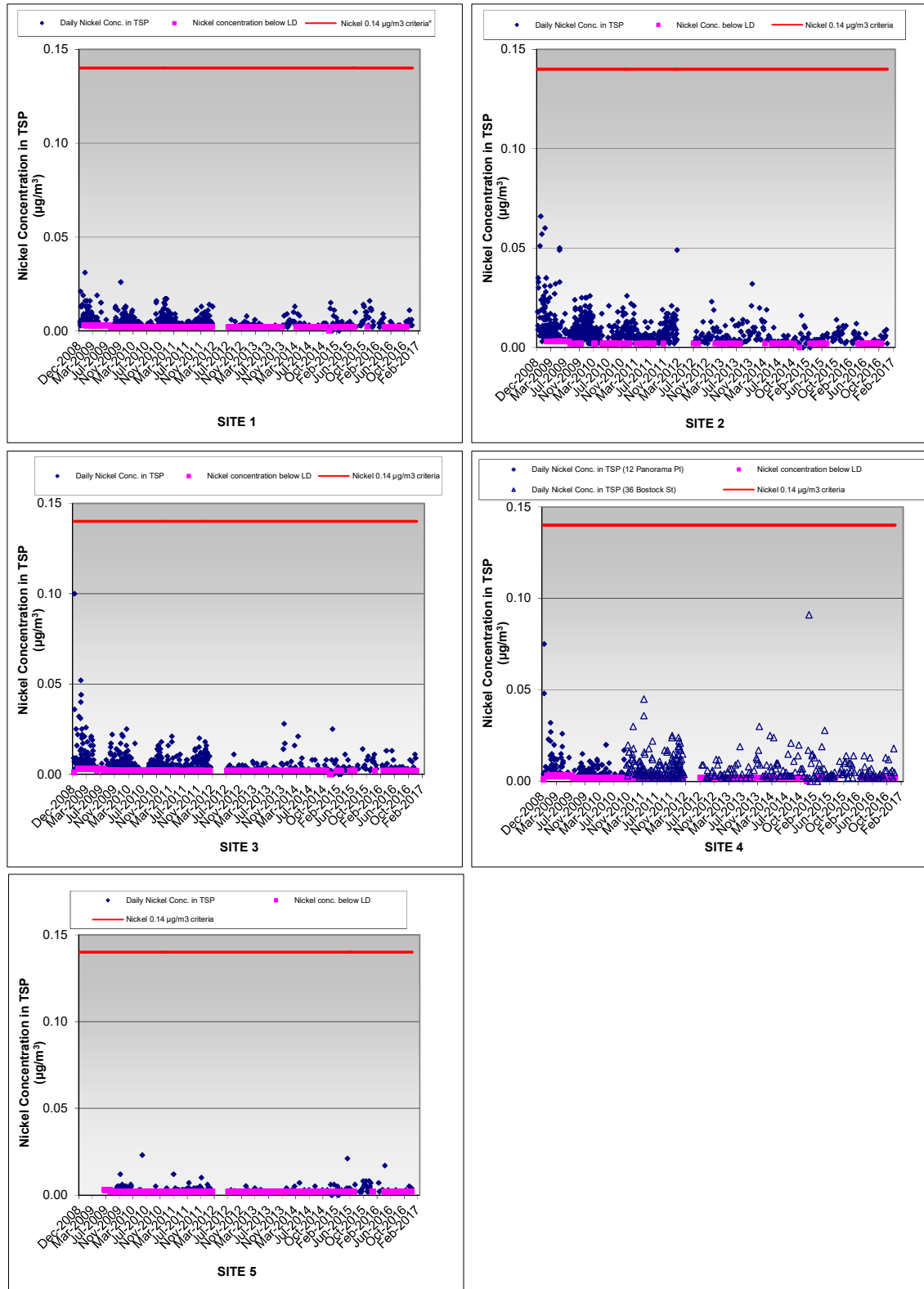
Figure 1: Concentrations of Nickel measured in Total Suspended Particulate (TSP) by High Volume Air Samplers (HVAS) at Sites 1 to 5 from 12 th December 2008 to 29 th December 2016
